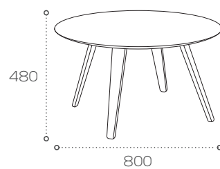
TAUC/RND0800FGL/BH4L
